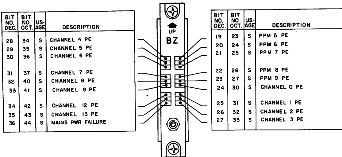
Figure 3-26. PPS-0 Module at 2D40 - Model 176
