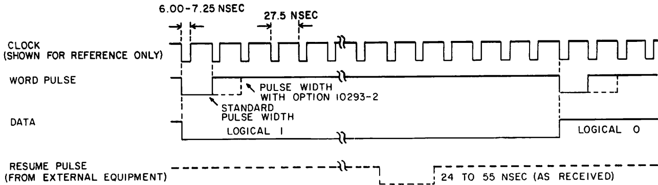
Figure 5-17. Output Channel Timing
