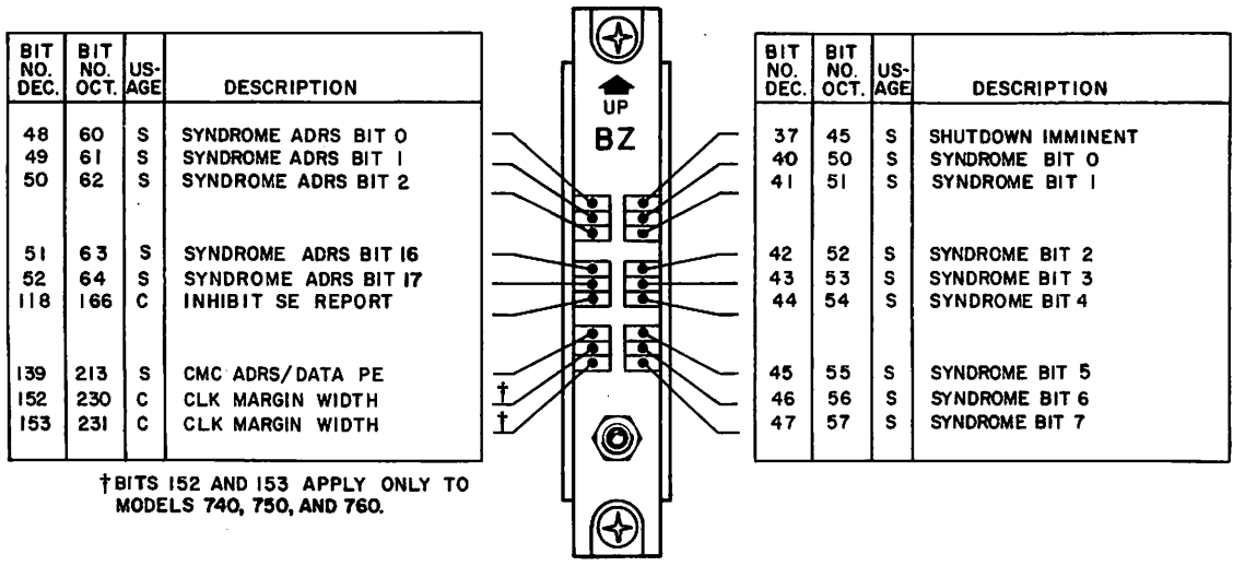
Figure 3-11. PPS-0 Module at 2B37 - Models 720 through 760
