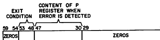
Figure 5-7. Format of Relative Address Zero on Error Exit - Models 720 through 760
