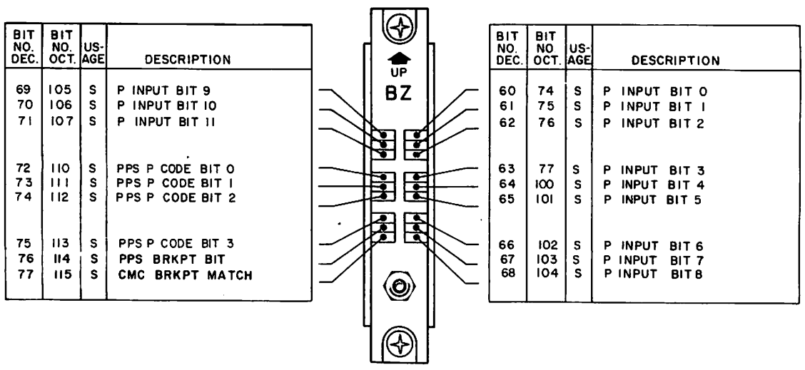
Figure 3-12. PPS-0 Module at 2C28 - Models 720 through 760
