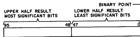
Figure 5-6. Multiply Result Format
