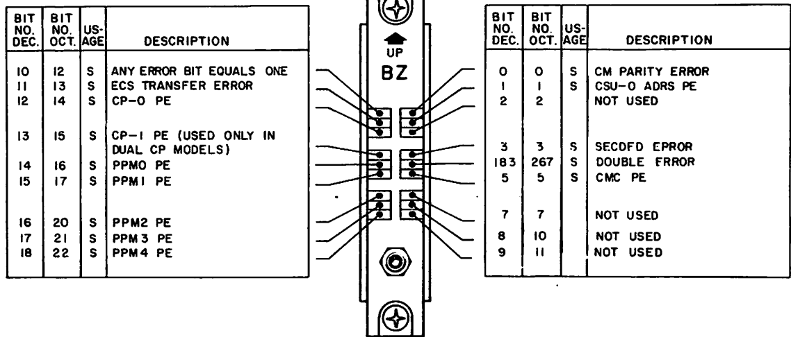
Figure 3-9. PPS-0 Module at 2C41 - Models 720 through 760
