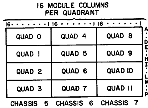
Figure 5-23. CP Chassis Quadrants (Viewed from Module Side) - Models 740, 750, and 760
